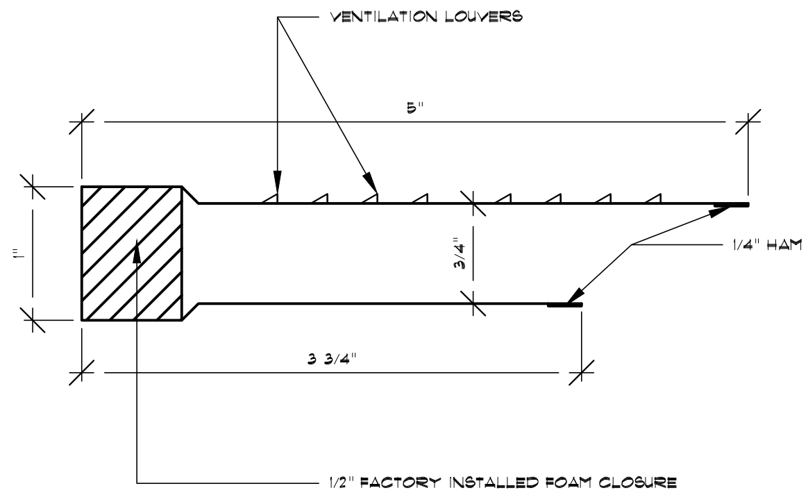
3/4" PROFILE
