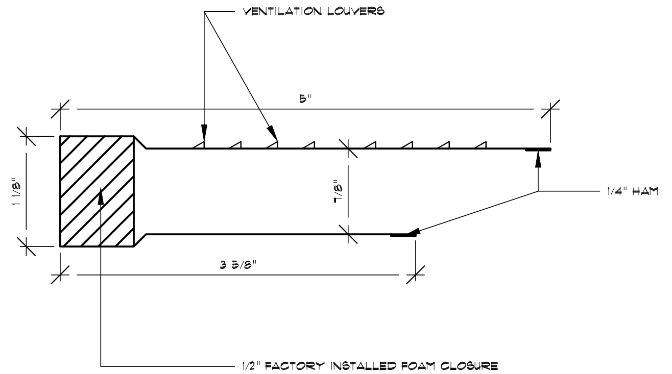
7/8" PROFILE
